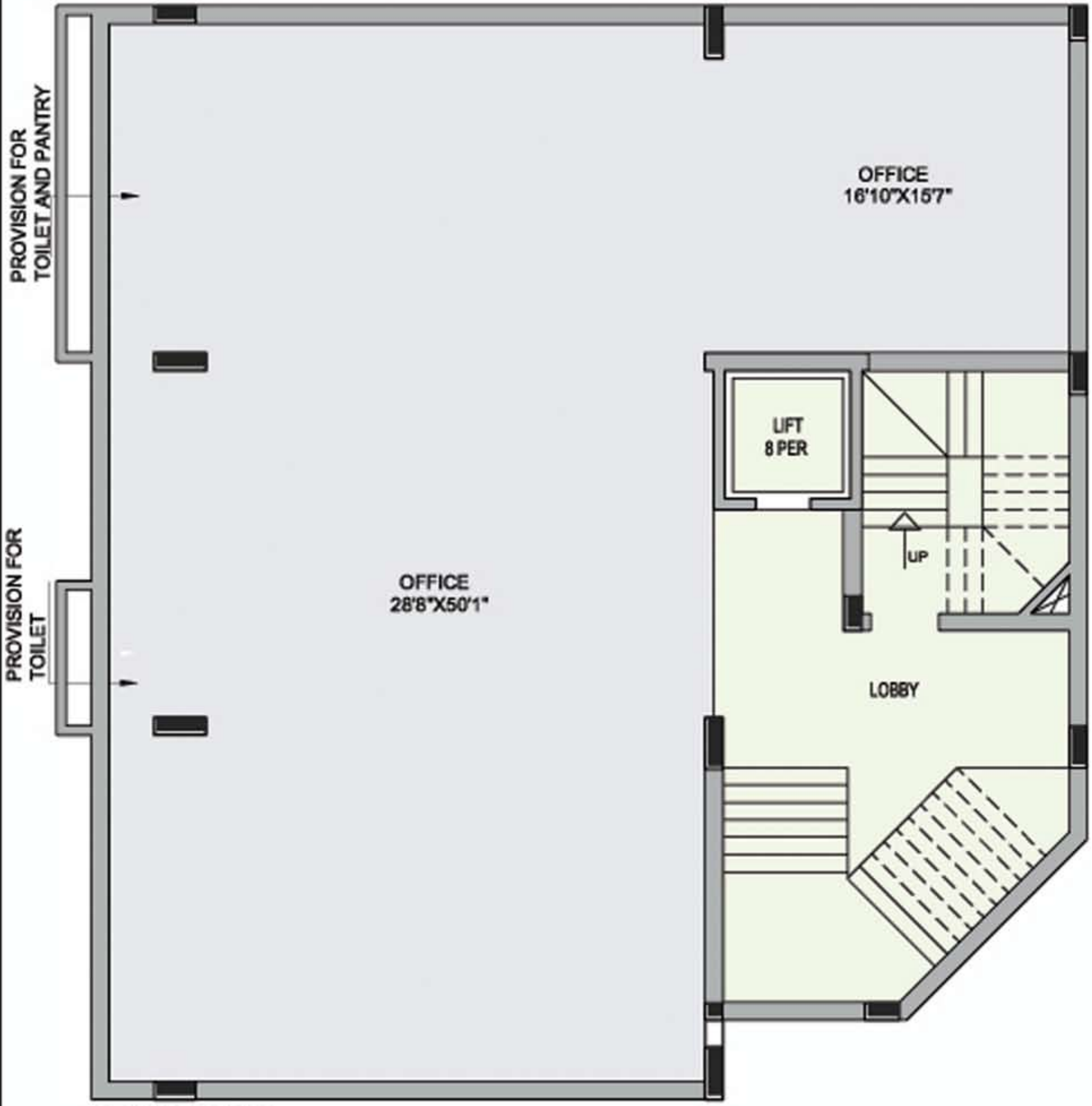
3rd FLOOR PLAN
